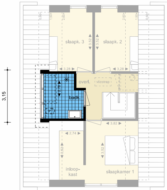
dakkapel type 4
